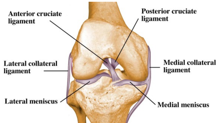
Figure 2.10: Ligaments of the knee joint [23]
