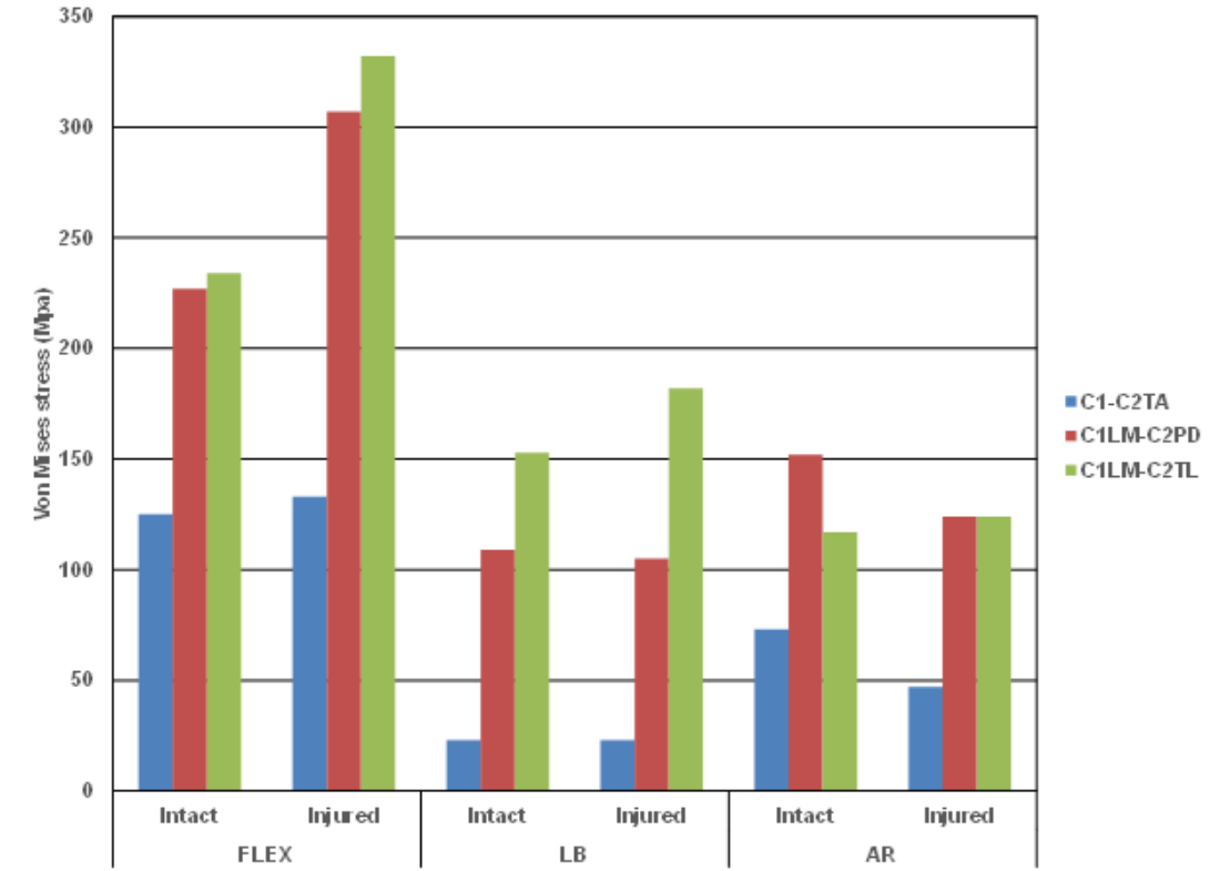
Figure 4.5: Maximum stress in the construct during FLEX, LB, and AR for both the intact and injured models
